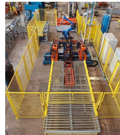
Gutter pipe Manufacturing Cell
